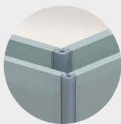
Detail 6600/42™ E (idem 6500/45™, 6600/48™, 6600/56™ en 6675/60™) Glaskoppeling hoek met CLIP-IN™ H-profiel
